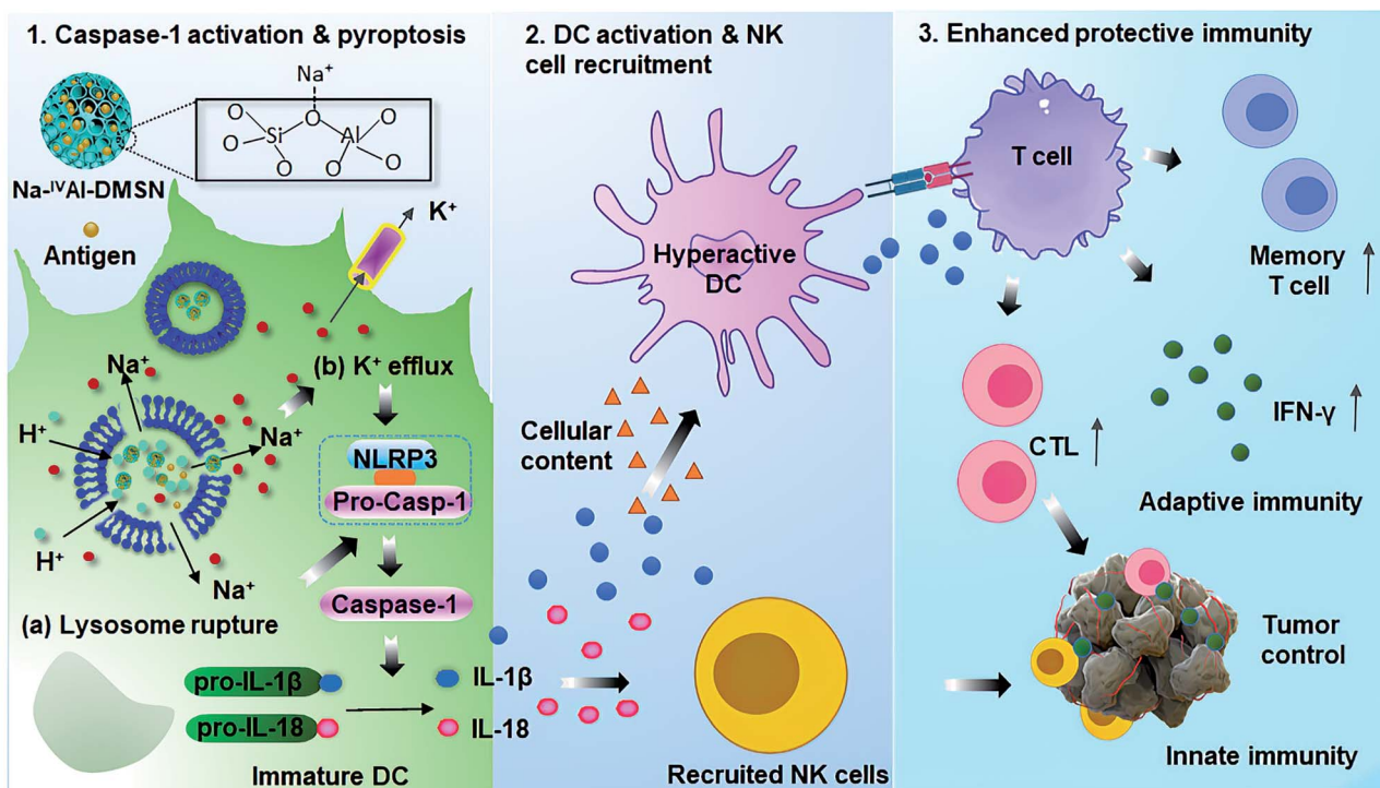
Scheme 1 Proposed mechanisms for \text{Na}^{\text{IV}}\text{Al-DMSN} induced DC pyroptosis and hyperactivation for enhanced innate immunity and adaptive immunity for tumor prophylaxis.
