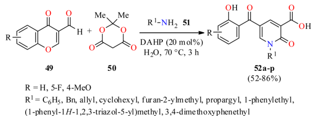
Scheme 14 DAHP-catalyzed three-component synthesis of 2-pyridone-3-carboxylic acids 52 and their in vitro antibacterial activity against four bacterial strains.
