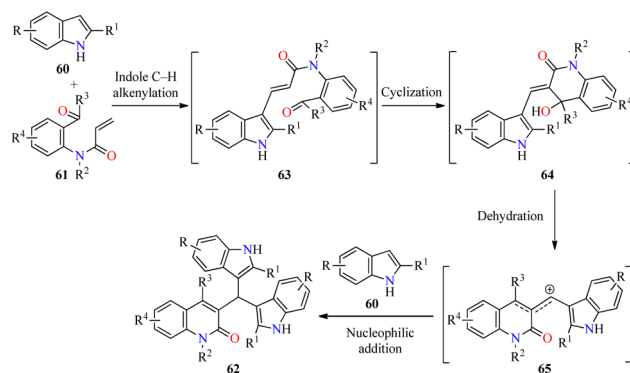
Scheme 18 Plausible mechanism for the synthesis of 3-bis(indol-3-yl)methylquinoline-2(1 H )-ones 62 .
