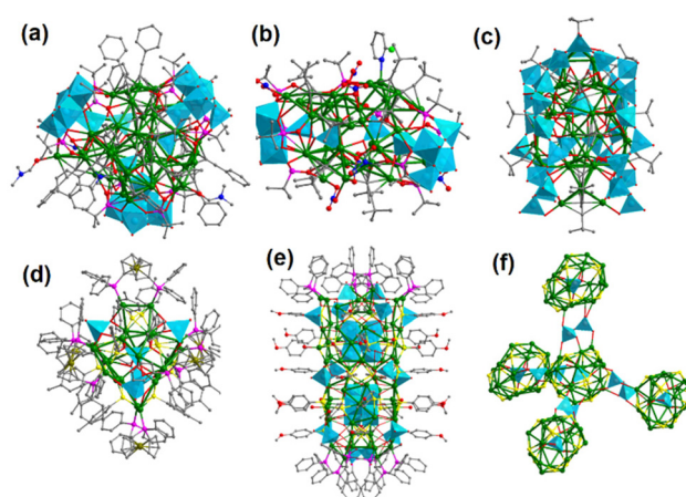
Fig. 18 Molecular structures of (a) [(O_2)V_2O_6]_3@Ag_{43} , (b) [(O_2)V_2O_6]_2@Ag_{36}[(^tBuPO_3)_4V_4O_8]_2 , (c) (V_2O_7)_2@Ag_{44}@(V_3O_9)_6 , (d) MoO_4@Ag_{24}@(MoO_4)_4 and (e) (Mo_6O_{22})_2@Ag_{76}@(MoO_4)_{16} . (f) Each CrO_4@Ag_{20} subunit connected to its adjacent four neighbours by Cr_2O_7^{2-} . (g) Molecular structure (left) and cyclic voltammogram (right) of SiW_{10}O_{37}@Ag_{41}-\beta-SiW_{12}O_{40} .
