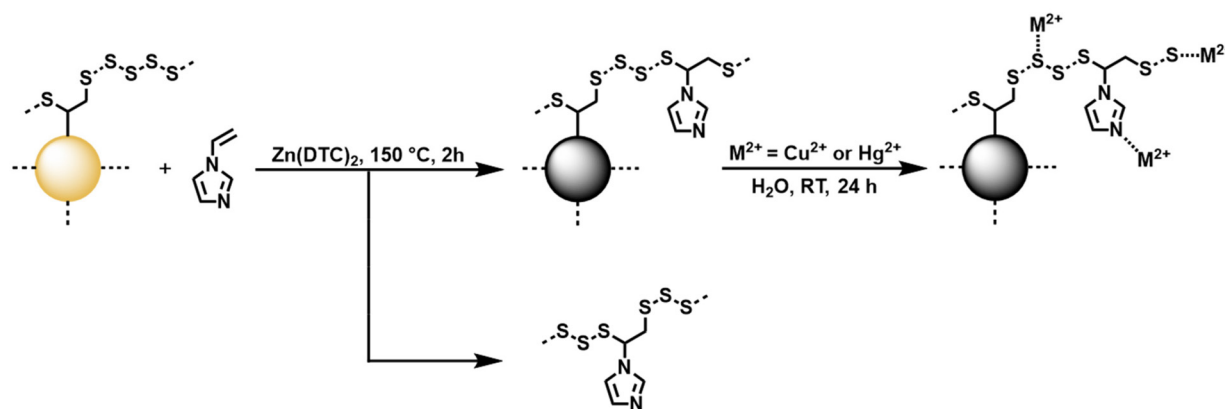
Scheme 2 Reaction equation of the dynamic covalent polymerization of inverse vulcanized TMVS-S particles with N -vinylimidazole to create TMVS-S-NVIA particles and their adsorption of Hg 2+ and Cu 2+ ions. Sulfur chains are abbreviated with dashed lines.
