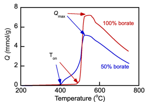
Fig. 6 CO 2 uptake by Li, Na borate (Li 1.5 Na 1.5 BO 3 ) and its eutectic Li, K carbonate (Li 1.24 K 0.76 CO 3 ) blend (borate/carbonate ratio, 1:1 mol/mol, sample no. 3 in Table 1) under 60 mL min -1 flow of 100% CO 2 at a heating rate of 0.33 °C min -1 . The CO 2 loading ( Q , mmol g -1 ) was calculated as a sample weight fraction ( 10 \times W_f ) gained on the exposure to the CO 2 flow, normalized by the molar mass of CO 2 (44.01 g mol -1 ). Arrows show the temperature datapoint at which the CO 2 uptake was measured to be at maximum ( Q_{max} ); T_{on} is the temperature of the CO 2 uptake onset. Numbers indicate nominal initial borate content.
