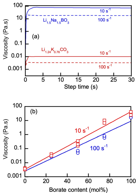
Fig. 5 (a) Rotational viscosity of Li, Na borate (Li 1.5 Na 1.5 BO 3 ) and eutectic Li, K carbonate (Li 1.24 K 0.76 CO 3 ) measured at 550 °C and at constant shear rates of 10 and 100 s -1 and the effect of borate concentration on viscosity of Li, Na borate (Li 1.5 Na 1.5 BO 3 ) and eutectic Li, K carbonate (Li 1.24 K 0.76 CO 3 ) blends at 550 °C and at shear rates of 10 and 100 s -1 (b). Numbers denote nominal initial borate concentration (mol%) in the blend. Straight exponent fits ( R^2 > 0.98 ) are shown to guide the eye only.
