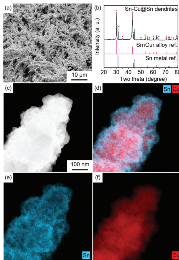
Fig. 1 Characterization of electrodeposited Sn-Cu@Sn dendrites. (a) SEM image and (b) XRD pattern. Reference patterns for Sn 7 Cu 1 alloy (PDF#03-065-3434) and Sn metal (PDF#00-004-0673) are displayed together. (c) HAADF-STEM image and (d) the corresponding EDS mapping image of Sn-Cu@Sn dendrites. Blue and red dots on the EDS map represent the signals from Sn and Cu, respectively. Single element distributions of (e) Sn and (f) Cu shown separately.
