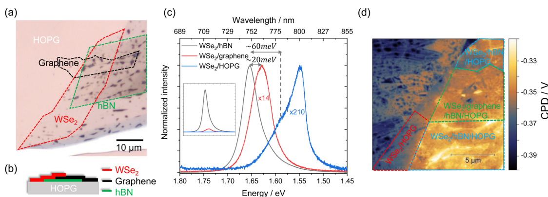
Fig. 4 (a) Optical microscopy image and (b) schematic cross-section of the \text{WSe}_2/\text{graphene}/\text{hBN}/\text{HOPG} hetero-stack. (c) PL spectra of \text{WSe}_2/\text{hBN} , \text{WSe}_2/\text{graphene} , and \text{WSe}_2/\text{HOPG} . For comparison, the intensities of the \text{WSe}_2/\text{graphene} and \text{WSe}_2/\text{HOPG} PL are normalized to that of \text{WSe}_2/\text{hBN}/\text{HOPG} . Inset: as-measured (not-normalized) PL spectra. (d) KPFM of \text{WSe}_2/\text{graphene}/\text{hBN}/\text{HOPG} .
