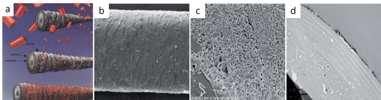
Fig. 7 Haloysite hair coating: the scheme of the process (a), SEM image of untreated human hair (b), and SEM (c) and TEM (d) cross-sectional images of the nanotube layer on hair. Adapted with permission from ref. 53 copyright by Royal Society of Chemistry, 2018.
