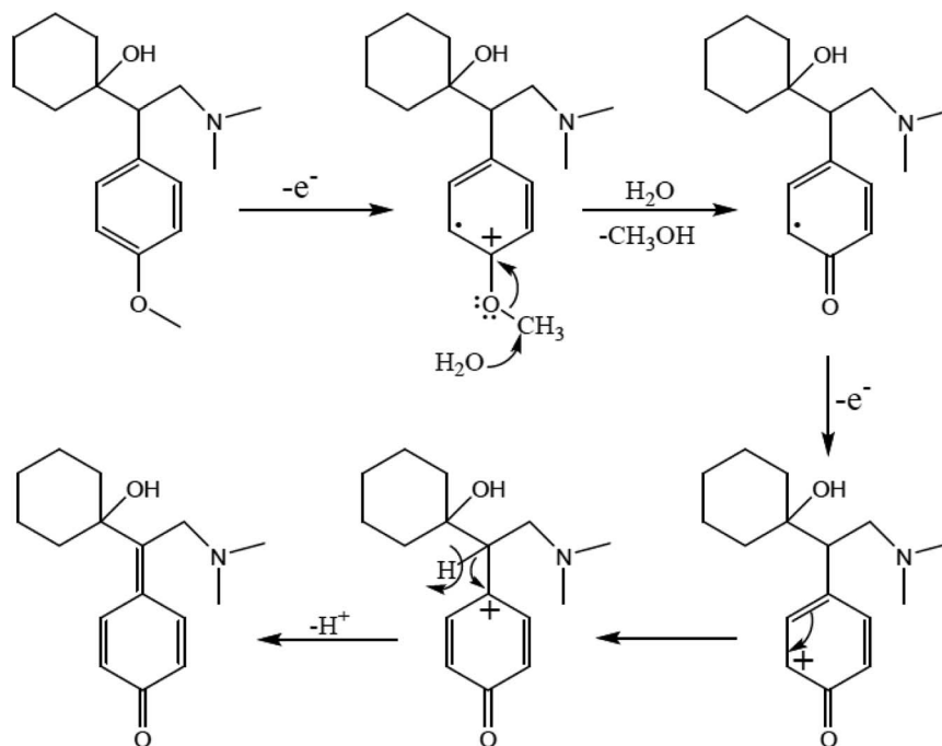
Fig. 28 Proposed mechanism for the electrooxidation of venlafaxine at the surface of Fe 3 O 4 @nano-cellulose/Cu nanocomposite/GSPE. This figure was adapted with permission from Industrial & Engineering Chemistry Research , 2020, 59, 4219–4228. 41
