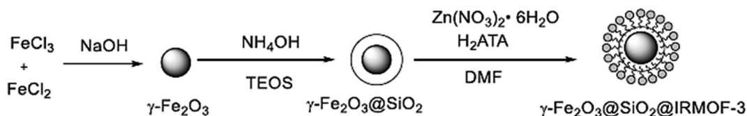
Fig. 29 Schematic showing the preparation of the γ-Fe 2 O 3 @SiO 2 /IRMOF-3 catalyst. This figure was adapted with a permission from Journal of Catalysis , 2020, 387, 39–46. 188
