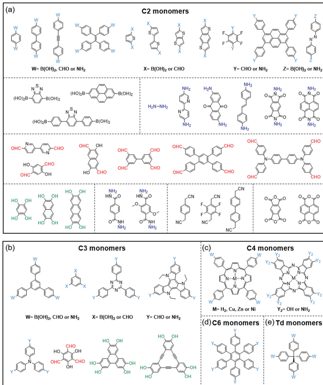
Fig. 1 Monomers with different geometries and reactive groups for the synthesis of COFs. The monomers can be divided into (a) C2, (b) C3, (c) C4, (d) C6 or (e) Td geometry.
