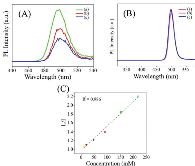
Fig. 2 (A) Delayed fluorescence emission spectrum of (a) Zn Au NCs and that following the addition of (b) 220 μL and (c) 560 μL addition of 1 M KI solution. (B) Prompt fluorescence emission spectrum of (a) Zn Au NCs and that following the addition of (b) 220 μL and (c) 560 μL addition of 1 M KI solution. (C) Stern Volmer plot calculated based on (A).
