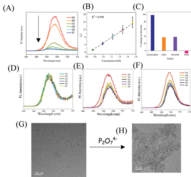
Fig. 3 (A) Emission spectrum of (a) Zn Au NCs and of those following the addition of (b) 15 μL, (c) 20 μL, (d) 25 μL, (e) 30 μL and (f) 35 μL of 100 mM of sodium pyrophosphate. (B) Corresponding Stern Volmer plot. (C) Bar diagram showing the percentage decrease in the luminescence intensity of Zn Au NCs upon the addition of pyrophosphate and various other interfering agents. (D) Emission spectrum of (a) Zn Au NCs and of those following the addition of (b) 20 μL, (c) 30 μL, (d) 40 μL, (e) 50 μL and (f) 60 μL of 100 mM of sodium nitrate. (E) Emission spectrum of (a) Zn Au NCs and of those following the addition of (b) 20 μL, (c) 30 μL, (d) 40 μL, (e) 50 μL and (f) 60 μL of 100 mM of sodium sulphate. (F) Emission spectrum of (a) Zn Au NCs and of those following the addition of (b) 20 μL, (c) 30 μL, (d) 40 μL, (e) 50 μL and (f) 60 μL of 100 mM of sodium thiosulphate. (G) Transmission electron microscopic image of Zn Au NCs and (H) of that following the addition of 30 μL of 100 mM sodium pyrophosphate.
