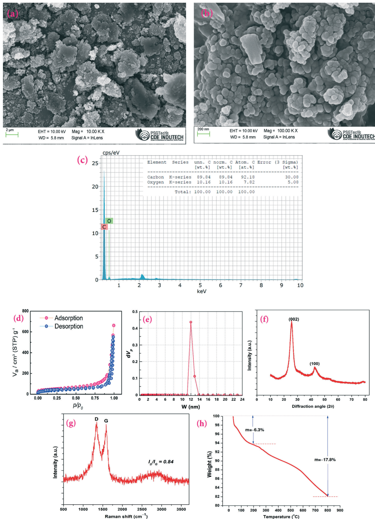
Fig. 3 Characterization of the produced CSCNP using SEM micrographs at magnifications of (a) 2 \mu\text{m} and (b) 200 \text{ nm} ; (c) EDX analysis showing the percentage of the elements present; (d) \text{N}_2 adsorption/desorption isotherm; (e) NLDFT/GCMC pore size distribution analysis; (f) XRD diffractogram; (g) Raman spectrum; and (h) thermogravimetric analysis.
