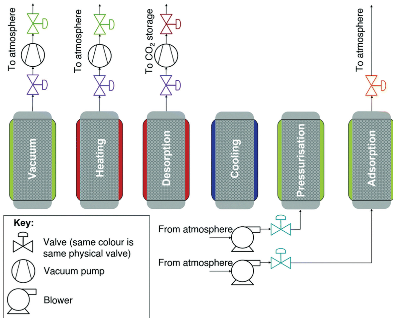
Fig. 15 A schematic of a simple temperature and vacuum swing DAC process. A full cycle includes evacuation of the adsorbent chamber, heating, a second heating step where \text{CO}_2 is extracted for storage, cooling to protect the sorbent from oxidative degradation, exposure to the atmosphere and adsorption. Reproduced from ref. 239 with permission from the Royal Society of Chemistry.
