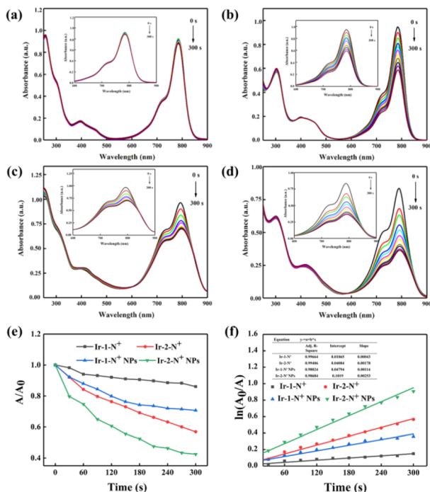
Fig. 4 The UV-vis absorption spectra of ICG ( 5 \mu\text{g mL}^{-1} ) with Ir-1-N + (a), Ir-2-N + (b), Ir-1-N + NPs (c) and Ir-2-N + NPs (d). (e) The decay rates of ICG in the presence of Ir-1-N and Ir-2-N and their NPs upon exposure to light illumination ( 425 \text{ nm} , 20 \text{ mW cm}^{-2} ). (f) Time-dependent ^1\text{O}_2 generation kinetics. A_0 = initial absorbance maximum of ICG. A = real-time absorbance maximum of ICG with various light exposure times. An enlarged inset table is shown as Table S2 in ESI.†
