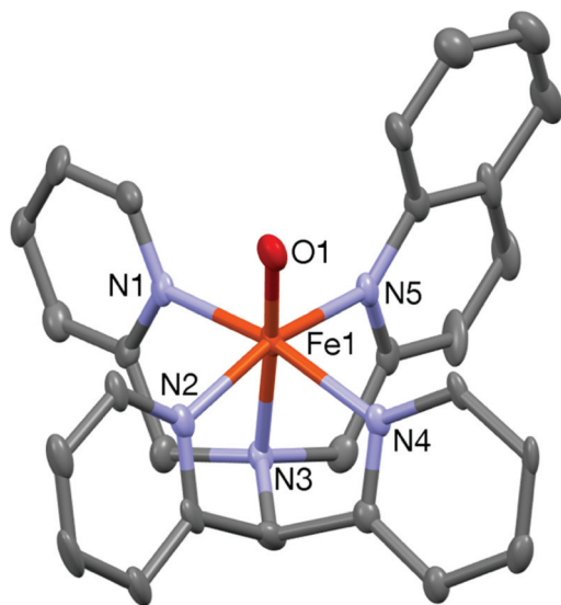
Fig. 6 A Mercury plot of the complex cation of 8 with 40% thermal ellipsoids. All hydrogen atoms have been omitted for clarity.
