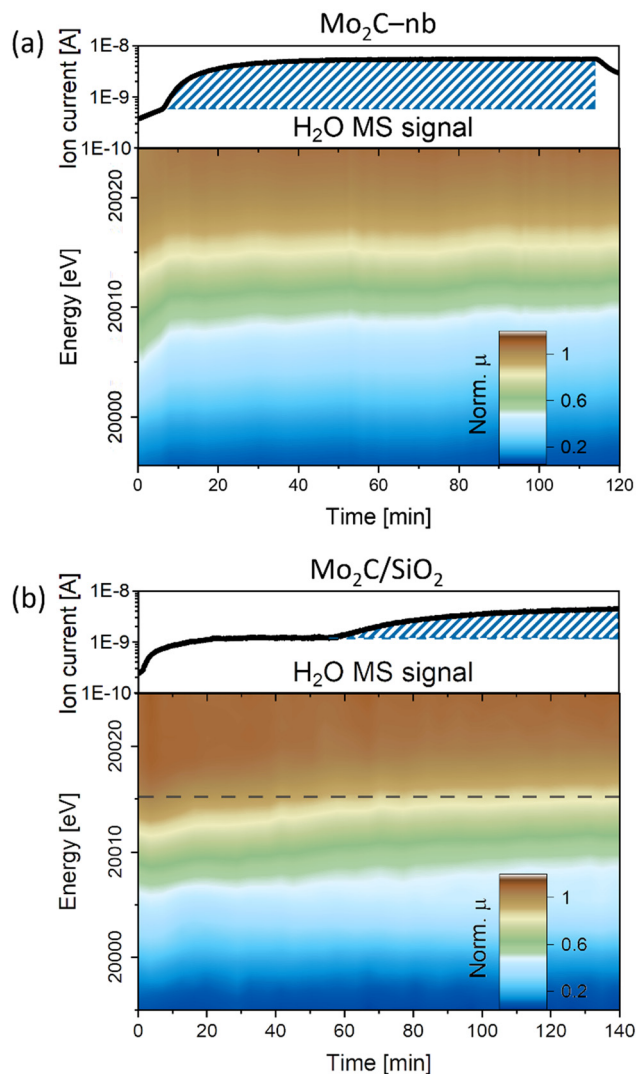
Fig. 3 In situ Mo K-edge XANES (contour plots of the intensity as a function of energy and time) during DRM (capillary reactor, 730 °C, 8 bar) of a) Mo 2 C-nb ( W/F = 45 ms g Mo mL -1 ) and b) Mo 2 C/SiO 2 ( W/F = 0.8 ms g Mo mL -1 ), complemented by the evolution of H 2 O MS signal.
