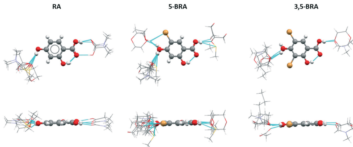
Fig. 3 First interaction shell with solvent of RA, 5-BRA and 3,5-BRA for all known crystal structures. Only hydrogen bonded solvent molecules are shown, solvent molecules are presented as wireframe for clarity.
