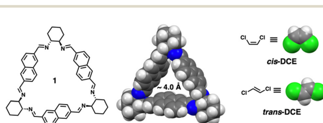
Scheme 1 Chemical structure of macrocycle 1 , cis - and trans -DCE.
