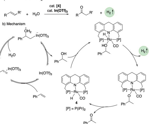
Fig. 21 (a) Alkene oxidation to a ketone with water catalyzed by 4. (b) Reaction mechanism.
