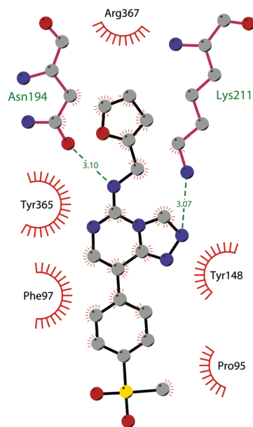
Fig. 14 Flat representation (generated using LigPlot+ from PDB ID 5GSA) showing contacts between compound 52 , EED, and an EZH2 peptide referred to as the EED binding domain (EBD). Hydrogen bonds are shown as dashed lines. The spoked arcs represent protein residues making non-bonded (hydrophobic) contacts with compound.
