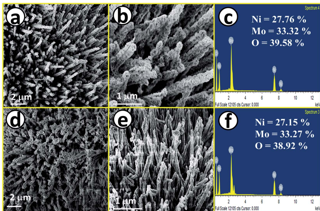
Fig. 2 (a) and (b) FE-SEM images of \text{NiMoO}_4 nano-rods, (c) EDS spectrum of \text{NiMoO}_4 in the FE-SEM mode, (d) and (e) FE-SEM images of \text{NiMoO}_4(\text{V}_6\text{O}_{13}) nanorod and (f) EDS spectrum of \text{NiMoO}_4(\text{V}_6\text{O}_{13}) in the FE-SEM mode.
