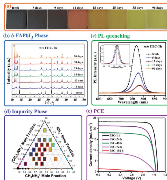
Fig. 11 (a) A series of photographs of perovskite films fabricated from perovskite precursor solutions aged for different amounts of time. The corresponding XRD (b) and PL spectra (c) of the perovskite films. Reprinted from ref. 130 with permission from Wiley. (d) Partial ternary phase diagram of [DMA] x (NH 4 ) y MA 1-x-y PbI 3 . Photographs of triple organic cation films are overlaid on the corresponding data points in the center of the phase diagram. Reprinted from ref. 106 with permission from the American Chemical Society. (e) I – V curves and distribution of the PCE of PSCs fabricated as a function of the aging time of the precursor solution. Reprinted from ref. 48 with permission from Wiley.
