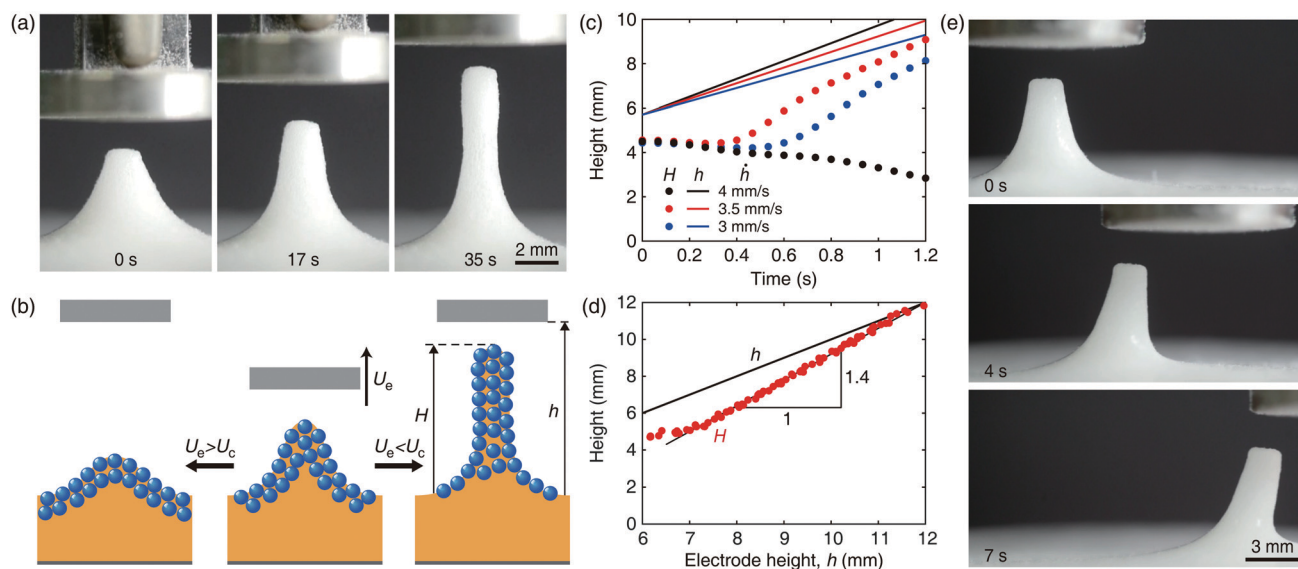
Fig. 3 Morphology control of the particle raft. (a) Images of a raft tower pulled vertically following the electrode that ascends from h = 6.4 to 10 \text{ mm} at a speed of 0.1 \text{ mm s}^{-1} . (b) Schematics of a particle raft that either collapses or grows depending on whether the electrode ascends at a speed higher or lower than the critical speed U_c . (c) Temporal evolution of the hill height (solid lines), which starts from H = 4.5 \text{ mm} with h = 5.7 \text{ mm} , for different ascent speeds of the electrode, U_e = 3, 3.5 , and 4 \text{ mm s}^{-1} . The particle raft grows upward following the electrode when the ascent speed is 3 and 3.5 \text{ mm s}^{-1} , but it collapses when U_e = 4 \text{ mm s}^{-1} . The dotted lines indicate the elevation of the electrodes, h . (d) The change of the raft height H as the electrode rises at U_e = 0.1 \text{ mm s}^{-1} . (e) Horizontal translation of a tower following the electrode horizontally moving at a speed of 2 \text{ mm s}^{-1} . In (a) and (c)–(e), the electric potential \phi is 10 \text{ kV} .
