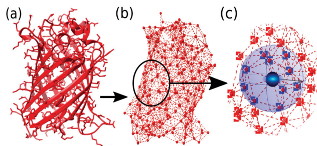
Fig. 2 Illustration of ANM using GFP protein (PDB code: 1W7S) from (a) starting PDB structure to (b) ANM representation at r_{\max} of 8 Å, (c) bonding criteria per residue: all particles within distance r_{\max} (bonds depicted by blue sphere) of center particle (black circle) are considered 'bonded' (blue squares) while those further (outside of sphere) are considered 'nonbonded' (red squares).
