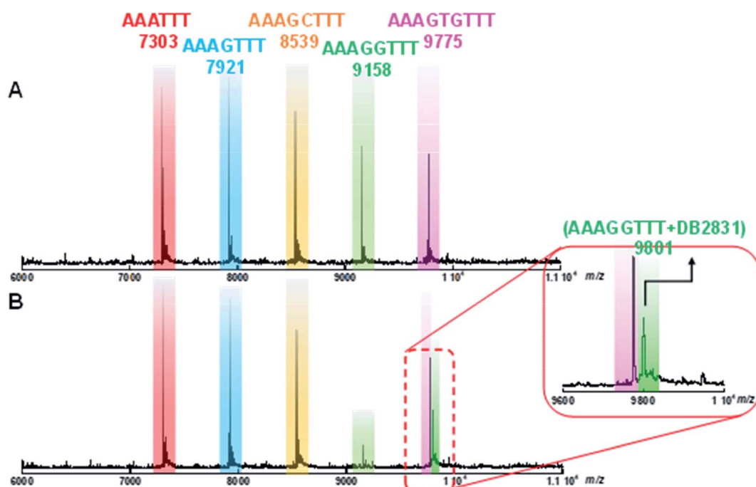
Fig. 5 ESI-MS negative mode spectra of the competition binding of sequences AAATTT; AAAGTTT; AAAGCTTT; AAAGGTTT; AAAGTGT: ( 10 \mu\text{M} each); with 40 \mu\text{M} DB2831 in buffer (50 mM ammonium acetate with 10% methanol (v/v), pH 6.8). (A) The ESI-MS spectra of free DNA mixture. (B) The ESI-MS spectra of DNA mixture with compounds. The ESI-MS results shown here are deconvoluted spectra and molecular weights are shown with each peak. The inset in red box is the expansion of (B) between 9600 and 10 000 m/z .
