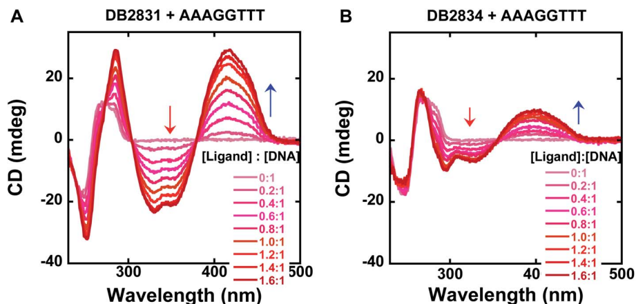
Fig. 4 Circular dichroism spectra for the titration of representative compounds, DB2831, DB2834 with a 5 \mu\text{M} AAAGGTTT sequence in TNE100 buffer at 25 \text{ }^\circ\text{C} . Arrows indicate the changes. Full DNA sequences as described in Fig. 1C.
