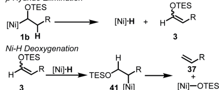
Scheme 2 Mechanistic considerations and catalytic cycle.
