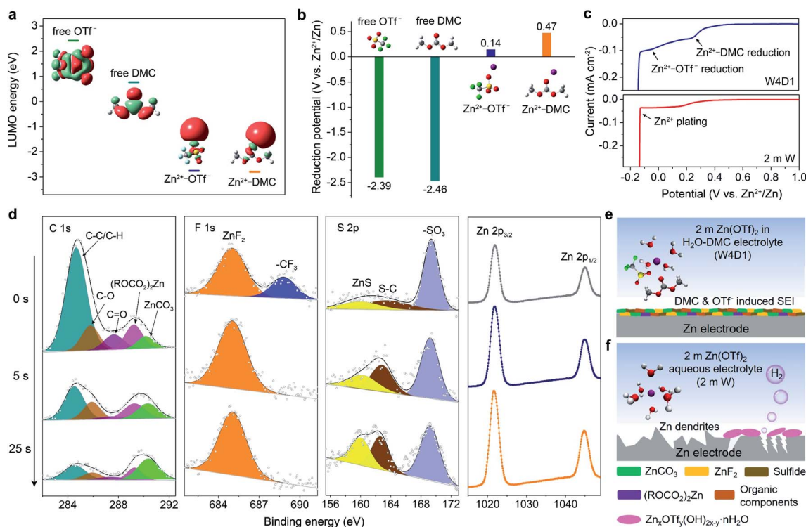
Fig. 5 SEI characterization on the Zn anode. (a) LUMO energy levels with corresponding LUMO isosurfaces and (b) the predicted reduction potential with geometric structures of the free OTf^- anion, free DMC solvent, and Zn^{2+} - OTf^- and Zn^{2+} -DMC coordinations from DFT calculations. (c) LSV profiles of W4D1 and 2 m W electrolytes at 5\text{ mV s}^{-1} . (d) XPS spectral regions for C 1s, F 1s, S 2p and Zn 2p with corresponding Ar^+ sputtering times on the Zn electrode in W4D1 after 10 cycles. Schematic illustration of the surface chemistry on the Zn electrode in (e) W4D1 and (f) 2 m W electrolytes.
