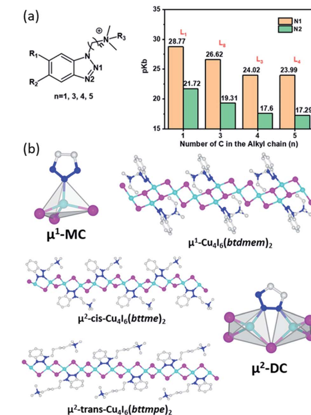
Fig. 2 (a) Ligand structures used to calculate \text{pK}_b values of N1 and N2 (left) and the calculated results in selected ligands with different alkyl chain length (right). Reproduced with permission from ref. 31. Copyright 2020, American Chemical Society. (b) Illustration of \mu^1\text{-MC} , \mu^2\text{-DC} modes and ligand orientations with representative hybrid structures. Color scheme: Cu, cyan; I, purple; N, blue; C, Gray.
