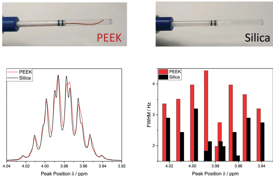
Fig. 3 Top: Photographs of a 1/32" OD (500 µm ID) PEEK injection capillary and a 0.8 mm OD (534 µm ID) fused silica injection capillary fitted to a Bruker InsightMR™ flow tube. Bottom: Comparison of ^1\text{H} NMR spectral quality and peak widths achievable at 500 MHz with a standard 'lctshim' routine on a sample of isopropanol flowing at 4 mL min ^{-1} at 20 °C using a peristaltic pump.
