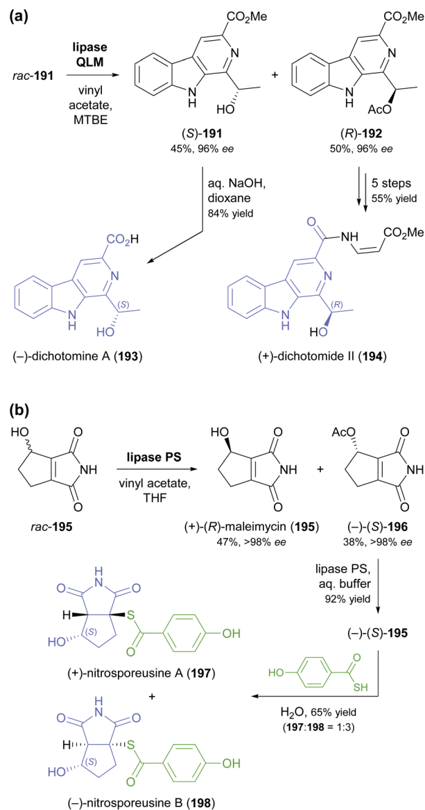
Scheme 23 Lipase-catalysed kinetic resolution of sec -alcohol moieties in alkaloids: (a) kinetic resolution of rac - 191 and its conversion into (-) -dichotomine A ( 193 ) and (+) -dichotomide II ( 194 ), (b) kinetic resolution of maleimycin ( 195 ) and its conversion into nitrosporeusines A and B ( 197 , 198 ).
