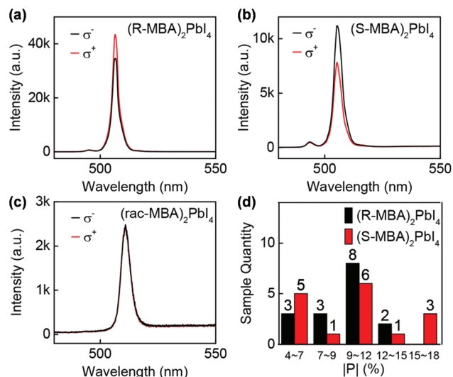
Fig. 6 (a–c) The circularly polarized PL spectra of (R\text{-MBA})_2\text{PbI}_4 , (S\text{-MBA})_2\text{PbI}_4 and (rac\text{-MBA})_2\text{PbI}_4 , respectively under excitation of 473 nm laser at 77 K. (d) Statistical histogram of the degree of CPL emission ( P ) for (R/S\text{-MBA})_2\text{PbI}_4 . This figure has been adapted/reproduced from ref. 70 with permission from American Chemical Society, Copyright 2019.
