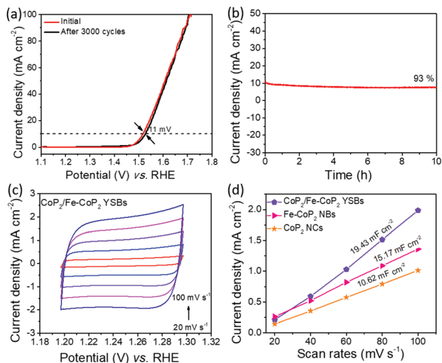
Fig. 8 (a) LSV curves of CoP 2 /Fe-CoP 2 YSBs before and after 3000 cycles. (b) Chronoamperometry stability test at a static potential of 1.50 V ( vs. RHE) for 10 hours. (c) Cyclic voltammery curves of CoP 2 /Fe-CoP 2 YSBs at different scan rates. (d) The capacitive current density as a function of scan rate for CoP 2 /Fe-CoP 2 YSBs, Fe-CoP 2 NBs and CoP 2 NCs. The measured double-layer capacitance of the system is taken as the average of the absolute value of the slope of linear fits to the data.
