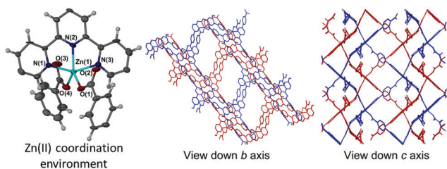
Fig. 2 Left: The zinc(II) coordination environment in 2 showing only the terpy region of the coordinating Hcbt ligand and coordinating benzoate groups of neighbouring Hcbt ligands. Ellipsoids are shown with 50% probability. Right: Stacked 2D sheets (shown in red and blue) of [\text{Zn}(\text{Hcbt})] in 2 as viewed down both the crystallographic b and c axes. Lattice solvents present within the channels have been removed for clarity.
