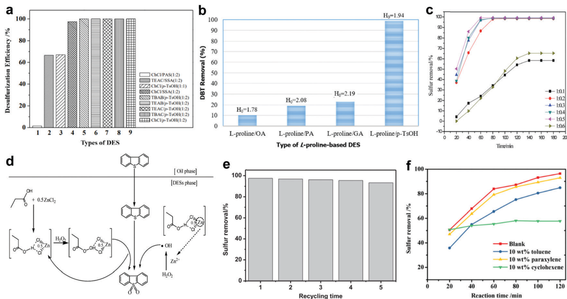
Fig. 9 (a) Catalytic activities of different DESs in oxidizing BT with \text{H}_2\text{O}_2 as oxidant at 25 °C in 1 h. Reprinted with permission. 118 Copyright 2015, Royal Society of Chemistry. (b) DBT removal efficiency and Hammett acidity function ( H_0 ) of different L-proline-based DESs in ODS system with \text{H}_2\text{O}_2 at 60 °C in 30 min. Reproduced with permission. 119 Copyright 2017, Elsevier B.V. (c) DBT removal efficiency using \text{C}_3\text{H}_6\text{O}_2/\text{XZnCl}_2 ( X = 0.1 to 0.6 ) and \text{H}_2\text{O}_2 at 40 °C in 1 h. (d) Reaction mechanism for oxidation of DBT using \text{C}_3\text{H}_6\text{O}_2/0.5\text{ZnCl}_2 as catalyst and extractant with \text{H}_2\text{O}_2 as oxidant. Reprinted with permission. 120 Copyright 2017, Royal Society of Chemistry. (e) DBT oxidation for five runs, at 3 h per run, using [PSTEtA]Cl/OA as catalyst and extractant at 50 °C in the presence of \text{H}_2\text{O}_2 . Reprinted with permission. 123 Copyright 2020, Elsevier B.V. (f) Effects of toluene, paraxylene and cyclohexene on the removal of DBT in the ODS system with ChCl/PEG/BA and \text{H}_2\text{O}_2 at 60 °C. Reprinted with permission. 124 Copyright 2019, Royal Society of Chemistry.
