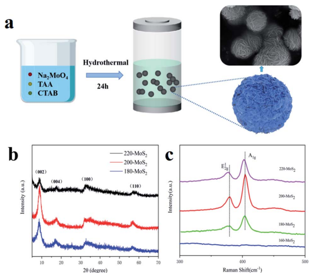
Fig. 1 (a) Schematic illustration of the preparation process of MoS 2 , (b) XRD of MoS 2 synthesized at different temperatures, (c) Raman spectra of MoS 2 synthesized at different temperatures.
