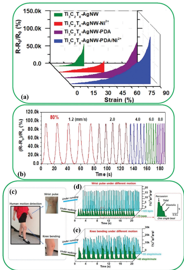
Fig. 15 (a) Typical relative resistance change vs. applied strain for the Ti_3C_2 -AgNW, Ti_3C_2 -AgNW- PDA , Ti_3C_2 -AgNW- Ni^{2+} , Ti_3C_2 -AgNW- PDA/Ni^{2+} strain sensors. (b) Relative resistance variation of the Ti_3C_2 -AgNW- PDA/Ni^{2+} strain sensor under incremental strain rates cycling from 0 to 80%. Monitoring human body (knee bonding and wrist pulse) under running and walking conditions by means of Ti_3C_2 -AgNW- PDA/Ni^{2+} strain sensors. (c) Images of wearable strain sensors attached to the wrist and knee. (d) Relative resistance variation of a wrist pulse. (e) Relative resistance change of knee bending. Reproduced with permission. 192 Copyright 2018, American Chemical Society.
