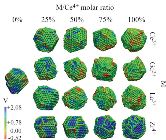
Fig. 10 Electrostatic potential map obtained with the particle-mesh Ewald method analysis for all nanoparticle structures at 0 K in relation to the M/Ce^{4+} ratio.
