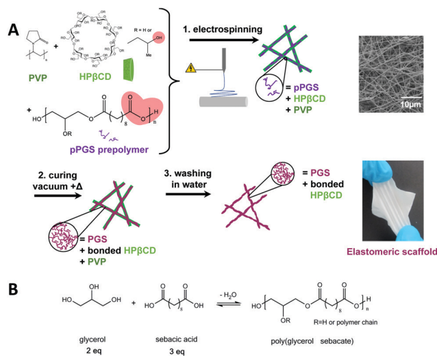
Fig. 1 Strategy for the elaboration of the elastomeric PGS-based fibers. During thermal treatment, pPGS is crosslinked and reaction of -\text{OH} groups of HP \beta CD with -\text{COOH} groups of pPGS (in red) occurs (A). Chemical scheme of pPGS synthesis by polycondensation of glycerol and sebacic acid (B).
