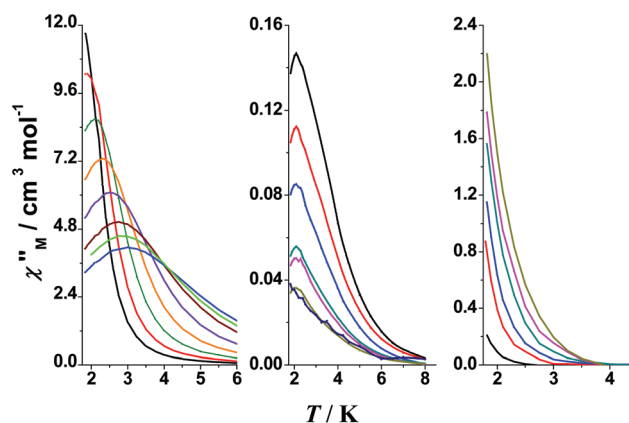
Fig. 8 (Left) \chi''_{\text{M}} vs. T signals for 1 in the 10–1488 Hz range at zero field; (middle) \chi''_{\text{M}} vs. T signals for 2 in the 1.45–148 Hz range under an applied dc field of 0.2 T; (right) \chi''_{\text{M}} vs. T signals for 3 in the 10–1488 Hz range at zero field. Solid lines are visual guides.
