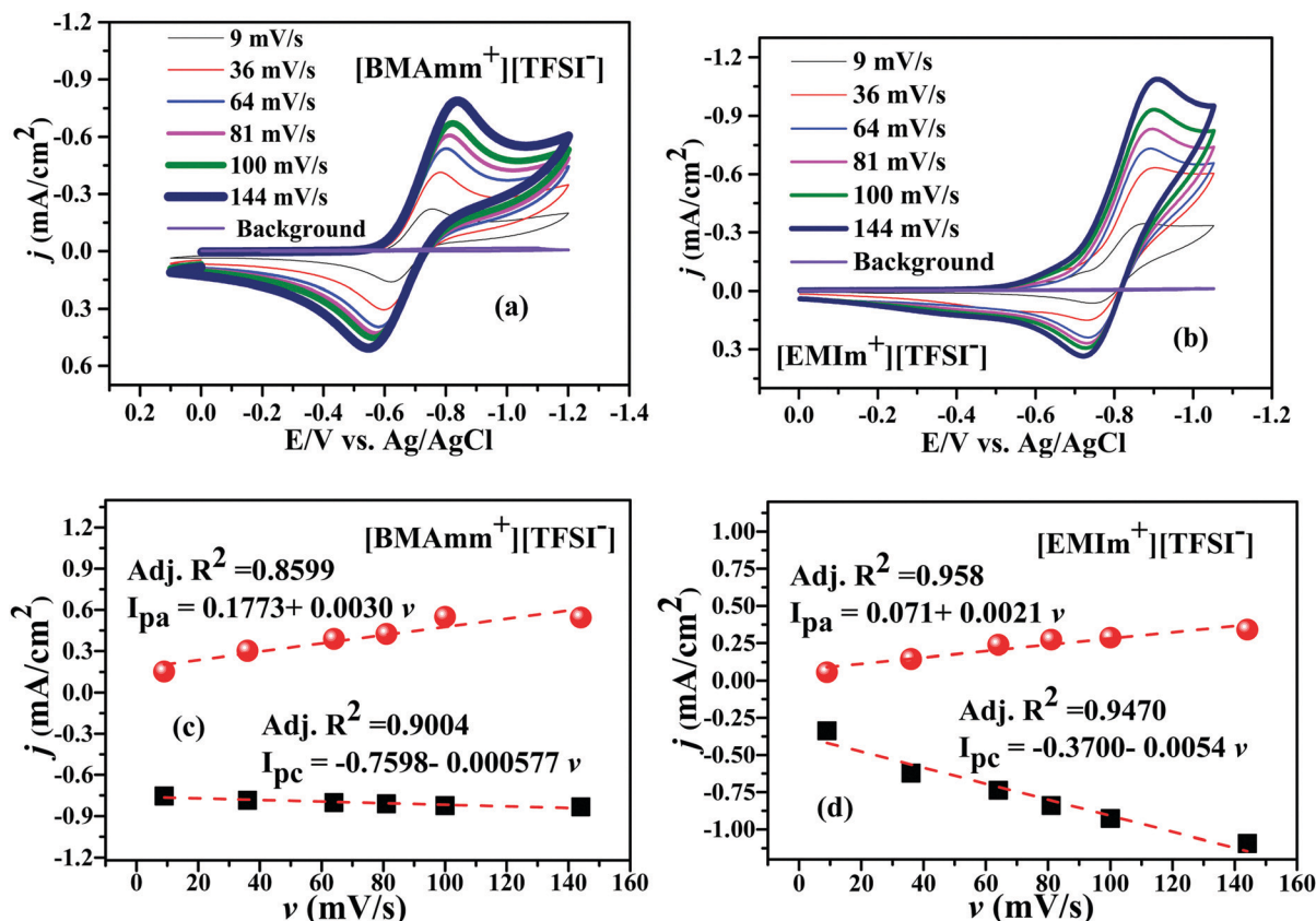
Fig. 3 CVs of O 2 •- generation in (a) [BMAMm + ][TFSI - ] and (b) [EMIm + ][TFSI - ], and current density against sweep rate in (c) [BMAMm + ][TFSI - ] and (d) [EMIm + ][TFSI - ].
