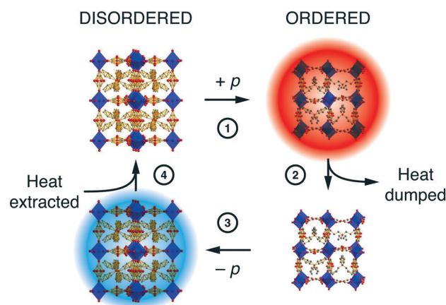
Fig. 5 A simple barocaloric cooling strategy that exploits the pressure-dependence of the order/disorder transition in [NPr 4 ][Mn(N(CN) 2 ) 3 ]. Starting at ambient conditions where the system is orientationally disordered (top left), ordering is induced by (1) application of pressure (note the change in unit cell dimensions is exaggerated here for effect). The loss of configurational entropy results in heating, and this excess heat (2) is dumped to the environment. (3) Removing the applied pressure forces the system to disorder; the concomitant increase in entropy now requires the system to cool. The cold solid (4) extracts heat from its environment. 74,75 Adapted from ref. 74 with permission from Springer Nature.
