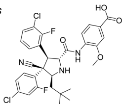
Idasanutlin (MDM2)
