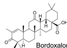
Bordoxalone (KEAP1)
