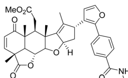
Nimbolide (RNF114)
