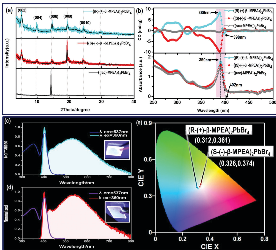
Fig. 2 (a) The XRD patterns of chiral perovskite crystals (R(+)-\beta\text{-MPEA})_2\text{PbBr}_4 , (S(-)-\beta\text{-MPEA})_2\text{PbBr}_4 film, (b) circular dichroism and steady-state absorption spectra of these perovskite crystals film. (c) PL and PLE spectra of (R(+)-\beta\text{-MPEA})_2\text{PbBr}_4 and (S(-)-\beta\text{-MPEA})_2\text{PbBr}_4 film ( \lambda_{ex} = 360\text{ nm} , \lambda_{em} = 537\text{ nm} ), (d) PL and PLE spectra of (S(-)-\beta\text{-MPEA})_2\text{PbBr}_4 and (S(-)-\beta\text{-MPEA})_2\text{PbBr}_4 film ( \lambda_{ex} = 360\text{ nm} , \lambda_{em} = 537\text{ nm} ), (e) CIE coordinated of the emissions of (R(+)-\beta\text{-MPEA})_2\text{PbBr}_4 and (S(-)-\beta\text{-MPEA})_2\text{PbBr}_4 film.
