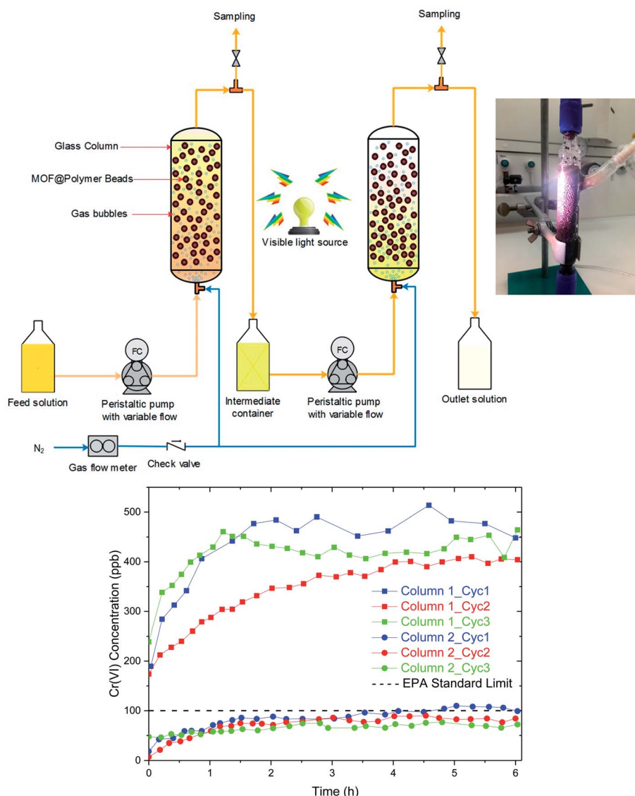
Fig. 5 (Top) The process flow diagram of the gas-sparged adsorption/photoreduction system (inset) column regeneration with HCl solution under irradiation (bottom) Cr(vi) concentration at the outlet of adsorption–photoreduction system (square) column 1 (circle) column 2 for three consecutive cycles.
