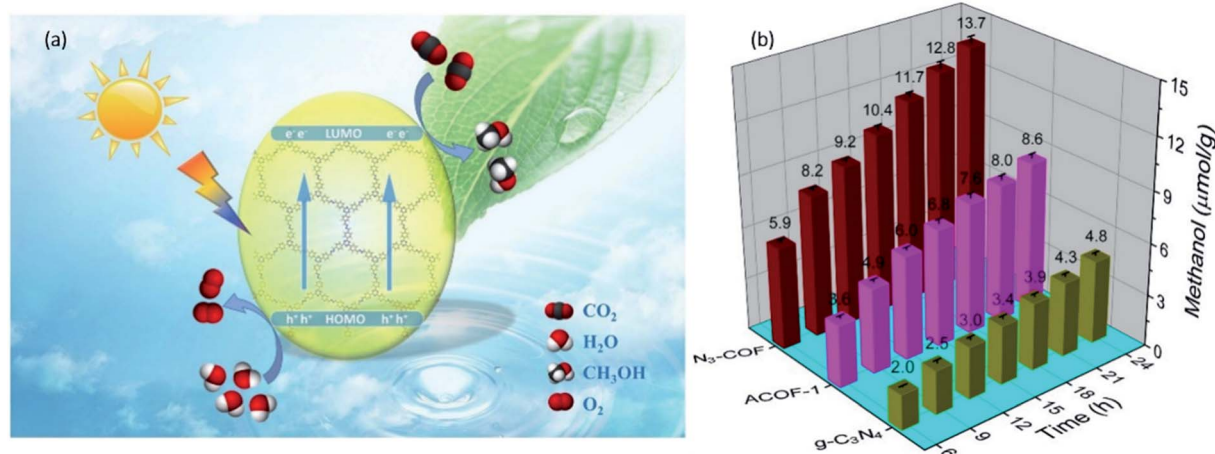
Fig. 11 (a) Schematic illustration for the photocatalytic reduction of \text{CO}_2 to \text{CH}_3\text{OH} over azine-based COFs. (b) Comparison of the amount of \text{CH}_3\text{OH} produced using ACOF-1, \text{N}_3\text{-COF} and \text{g-C}_3\text{N}_4 as the photocatalysts. Adapted with permission from ref. 88. Copyright 2018, Elsevier B.V.
