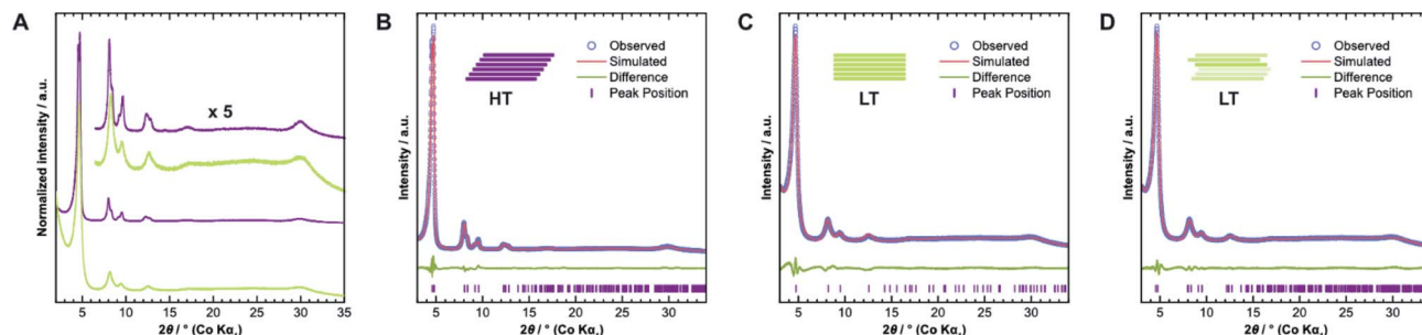
Fig. 4 (A) Comparison of X-ray diffraction patterns of HT (purple) and LT (green) collected with \text{Co K}\alpha_1 radiation. (B) Diffraction pattern of HT with best-obtained fit by Rietveld refinement assuming unidirectional slip stacking. (C) Diffraction pattern of LT with best-obtained fit by Rietveld refinement assuming eclipsed stacking and (D) random stacking.
