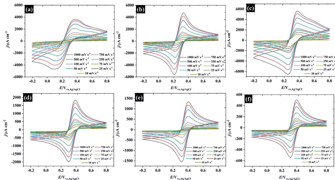
Fig. 3 CVs recorded using 10 \text{ mM K}_3\text{Fe}(\text{CN})_6 in potassium fluoride as a supporting electrolyte on an HOPG working electrode. KF concentrations are: (a) 0.5 \text{ M} , (b) 1.0 \text{ M} , (c) 5.0 \text{ M} , (d) 10 \text{ M} , (e) 13 \text{ M} , and (f) 17 \text{ M} .
