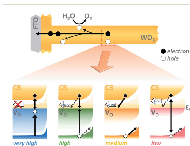
Scheme 1 (Upper) Illustration of a single nanoneedle of \text{WO}_3 (yellow) on FTO (grey), indicating electron (black arrows) transport (black arrows) and possible recombination pathways with holes (white) on route to extraction. (Lower) Indication of the dominant kinetic pathways immediately following charge separation in each of the samples examined; ‘very high’ [\text{V}_{\text{O}}] (left, blue), ‘high’ [\text{V}_{\text{O}}] (centre left, green), ‘medium’ [\text{V}_{\text{O}}] (centre right, yellow) and ‘low’ [\text{V}_{\text{O}}] (right, red). Arrow weight depicts likelihood of event. Filled \text{V}_{\text{O}} states are given in colour, empty states able to trap electrons are given in yellow. ‘Very high’ [\text{V}_{\text{O}}] shows hole trapping faster than instrument detection (heavy arrow). The ‘high’ doped sample has the greatest bulk trap recombination, particularly from hole trapping, so later carrier collection is limited. With too few defect states (‘low’, red), charge separation is hindered and the probability of geminate and bimolecular recombination increases. The best performing sample has the optimal amount of defects to aid charge separation without losing carriers to trap-mediated recombination.
