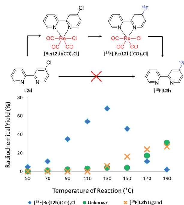
Fig. 4 RCYs of [\text{Re}(\text{L2h})(\text{CO})_3\text{Cl}] (blue diamonds), [\text{Re}(\text{L2h})(\text{CO})_3\text{Cl}] (orange crosses) and an unknown by-product (green circles) plotted as a function of the reaction temperature for the [\text{Re}(\text{CO})_3(\text{L2d})\text{Cl}] complex. [\text{Re}(\text{L2h})(\text{CO})_3\text{Cl}] was unable to be synthesised from L2d unless mediated by rhenium(i) complexation as per the above scheme.
