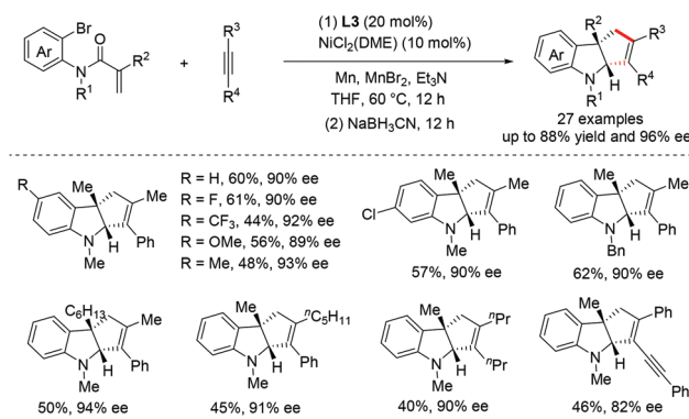
Scheme 11 Ni-Catalyzed enantioselective reductive cyclization of alkynes with arylbromide-tethered acrylamides.
